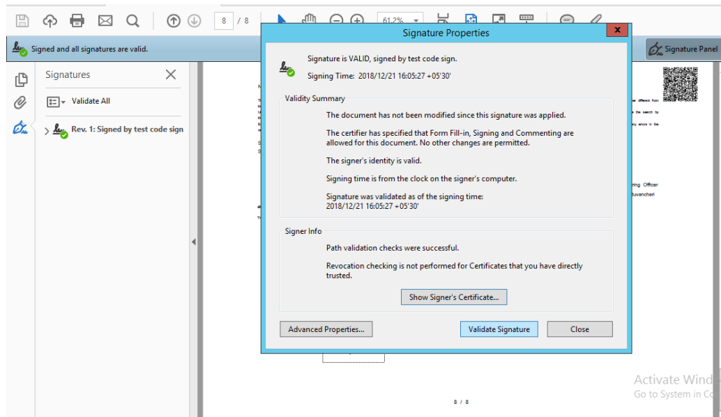
Figure 15: Validate Signature
