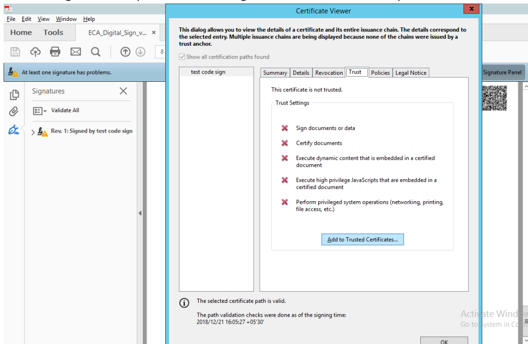
Figure 14: Certificate Viewer
