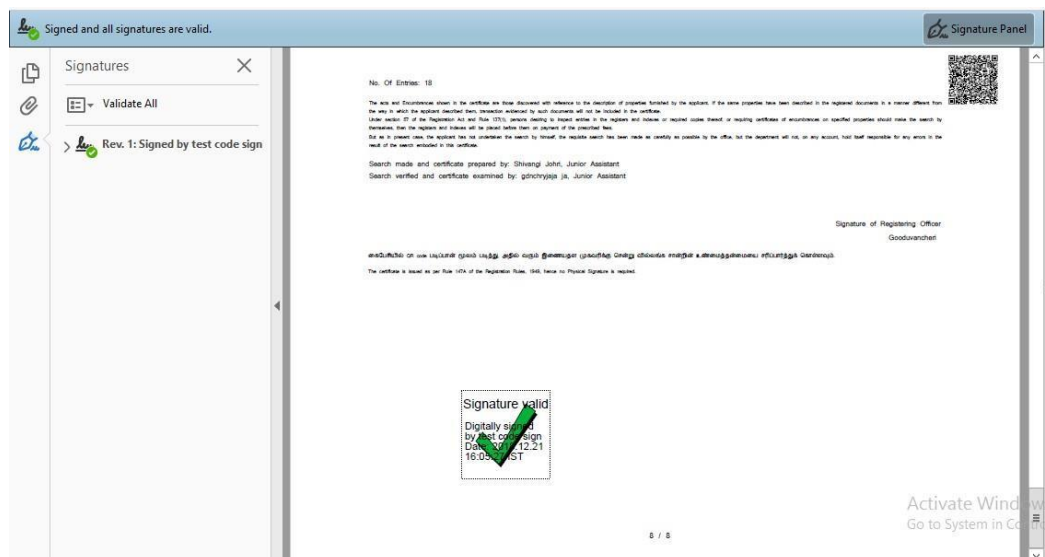
Figure 16: Validated Signature
